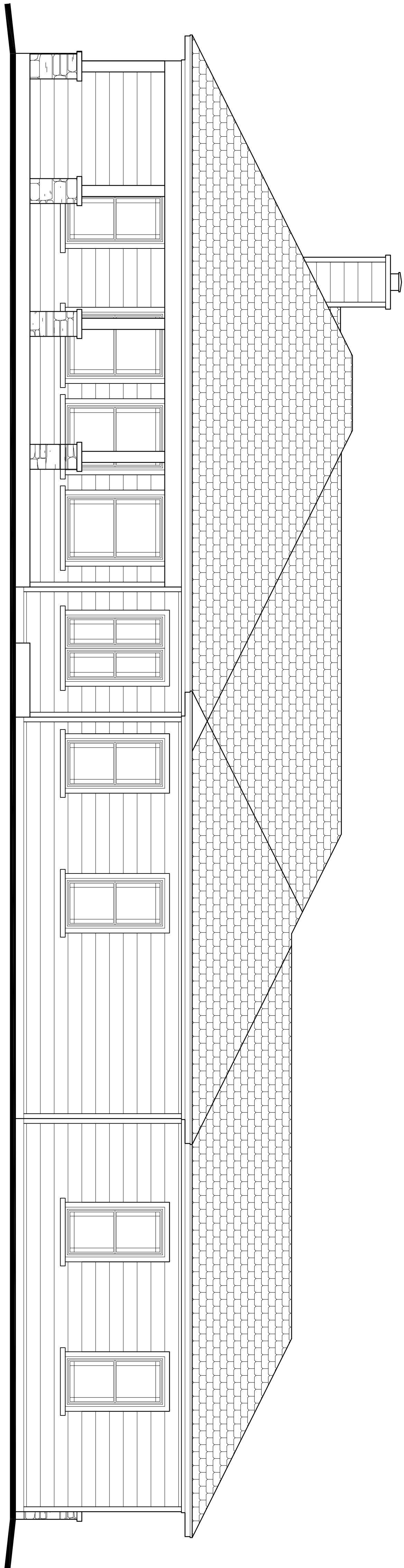
BACK ELEVATION
