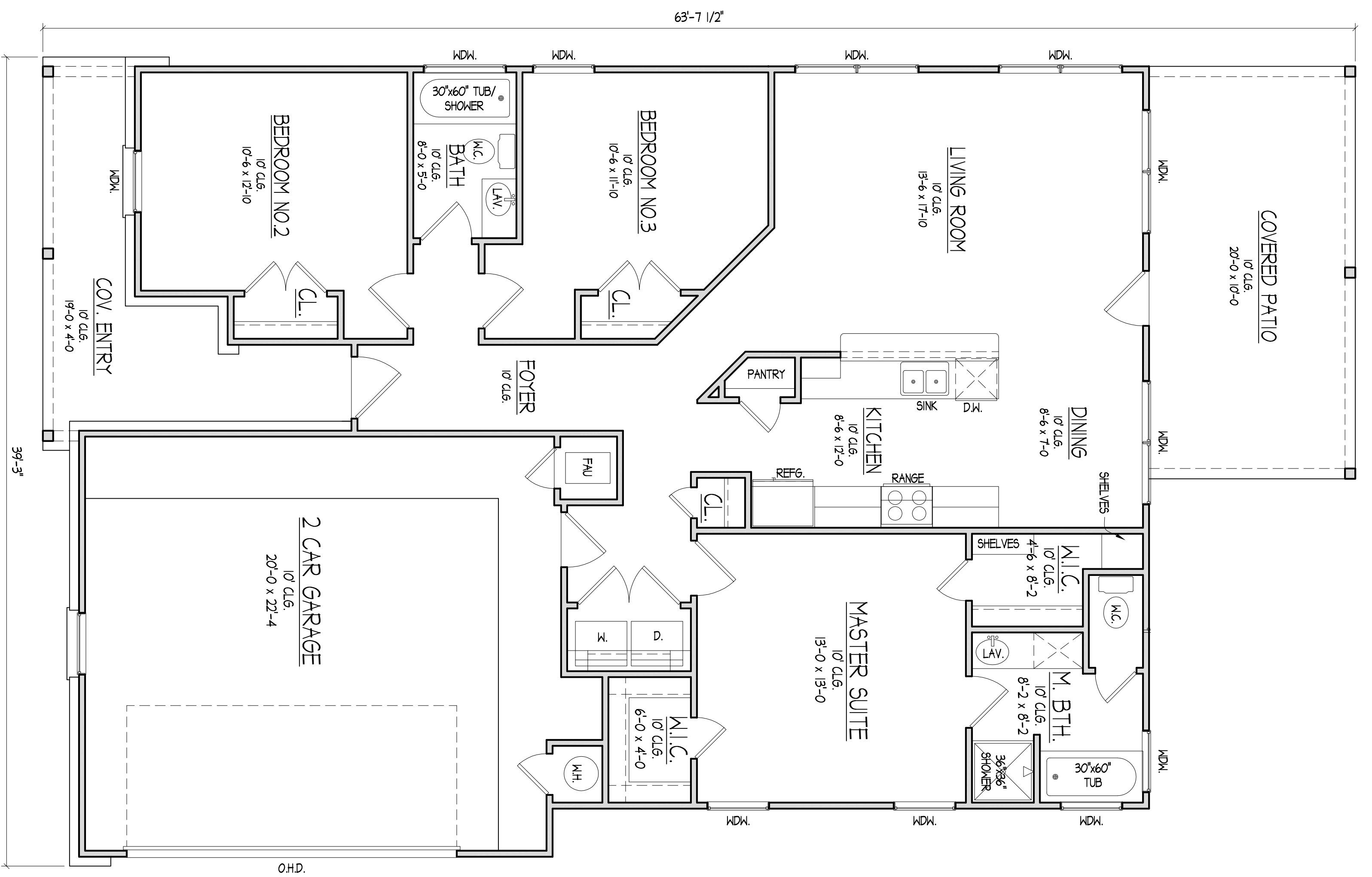
FLOOR PLAN
